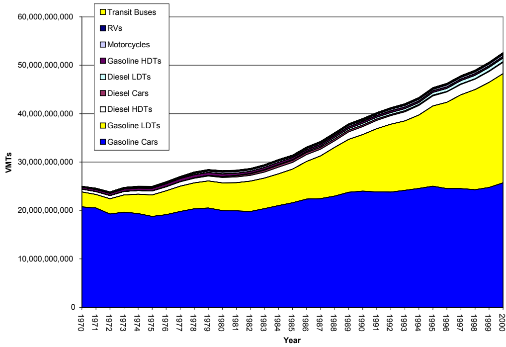
Figure 5.7 Vehicle Miles Traveled on Minnesota Highways
