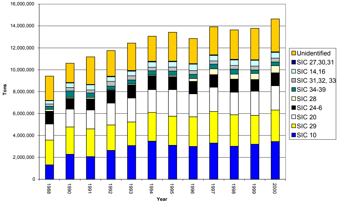
Figure 5.67 CO 2 Emissions from the Industrial Sector by Standard Industrial Classification Code
