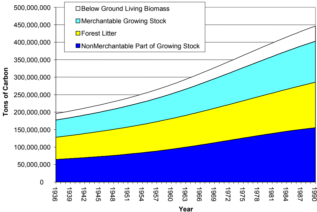
Figure 5.70 Carbon Storage on Minnesota Timberlands
