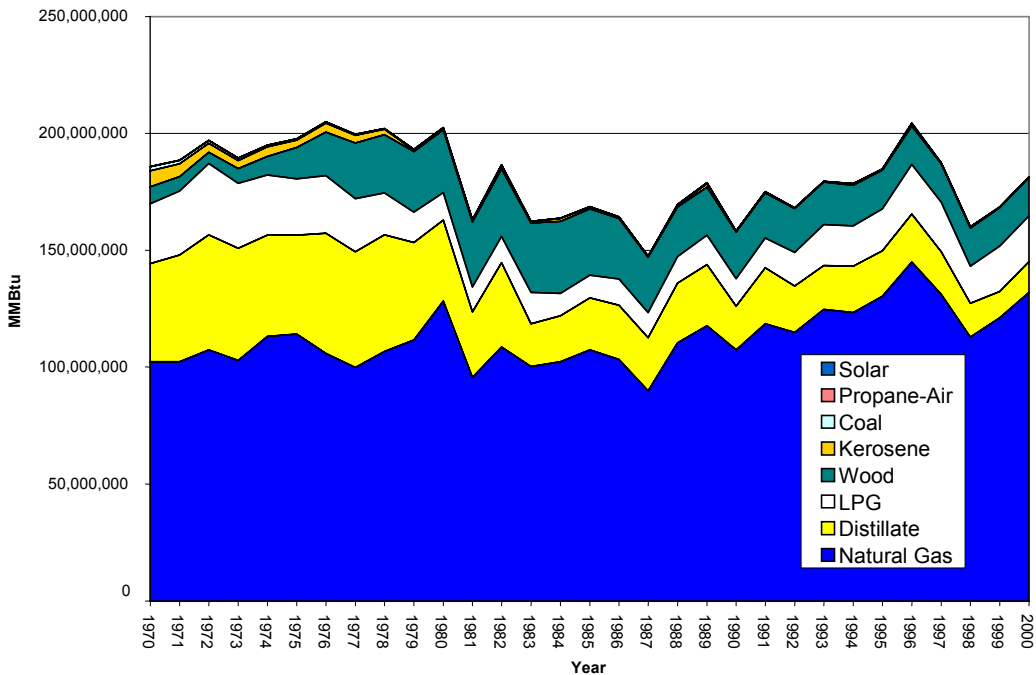
Figure 5.42 Nonelectric Energy Use in the Minnesota Residential Sector
