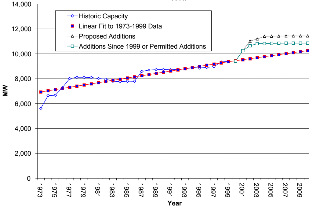
Figure 5.25 Historic and Forecasted Installed Summer Electricity Generation Capacity in Minnesota
