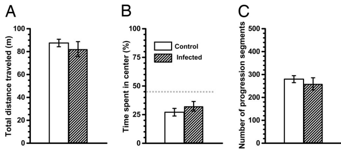
Fig. 4. Infection did not affect anxiety-like behavior of rats in the open-field arena. Control, n = 15 ; infected, n = 15 . Ordinates depict the total distance traveled during a 30-min trial (A), time spent in the center (inner two-thirds of the arena; the dotted line represents the chance level) relative to the total duration of the trial (B), and the number of progression segments (C).
