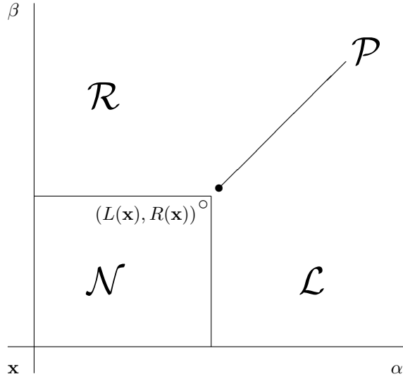
Figure 1: This figure illustrates the outcome classes of the game \alpha\mathbf{x}\beta for all ordinals \alpha and \beta . The unfilled circle represents the triple point, (L(\mathbf{x}), R(\mathbf{x})) , which has an outcome class of \mathcal{N} . The filled circle is the point (L(\mathbf{x}) + 1, R(\mathbf{x}) + 1) and the games on the line originating from the filled circle, which are of the form (L(\mathbf{x}) + \gamma, R(\mathbf{x}) + \gamma) where \gamma > 0 , have an outcome class of \mathcal{P} .
